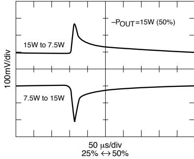
SMTR2815D +VOUT STEP LOAD RESPONSE
