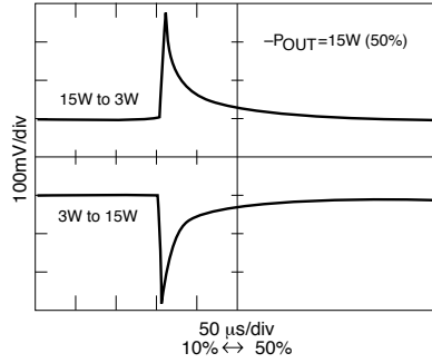
SMTR2815D +VOUT STEP LOAD RESPONSE
