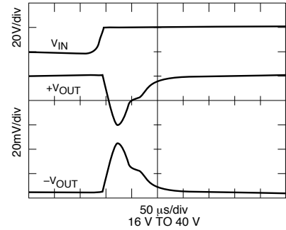
SMTR2815D STEP LINE RESPONSE
