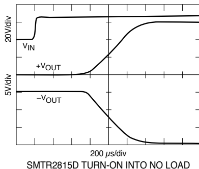
SMTR2815D TURN-ON INTO NO LOAD
