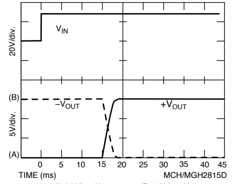
Also representative of MCH/MGH2812S & D and MCH/MGH2815S TURN-ON INTO FULL LOAD
