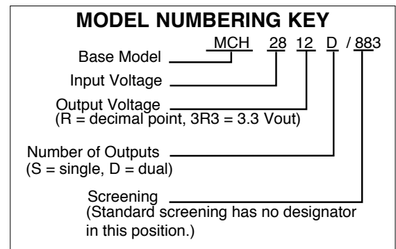
FIGURE 3: MCH MODEL NUMBERING KEY
