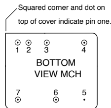
FIGURE 2: MCH PIN OUT
